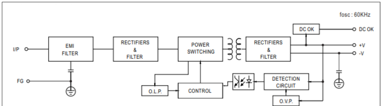
Functional Diagram
